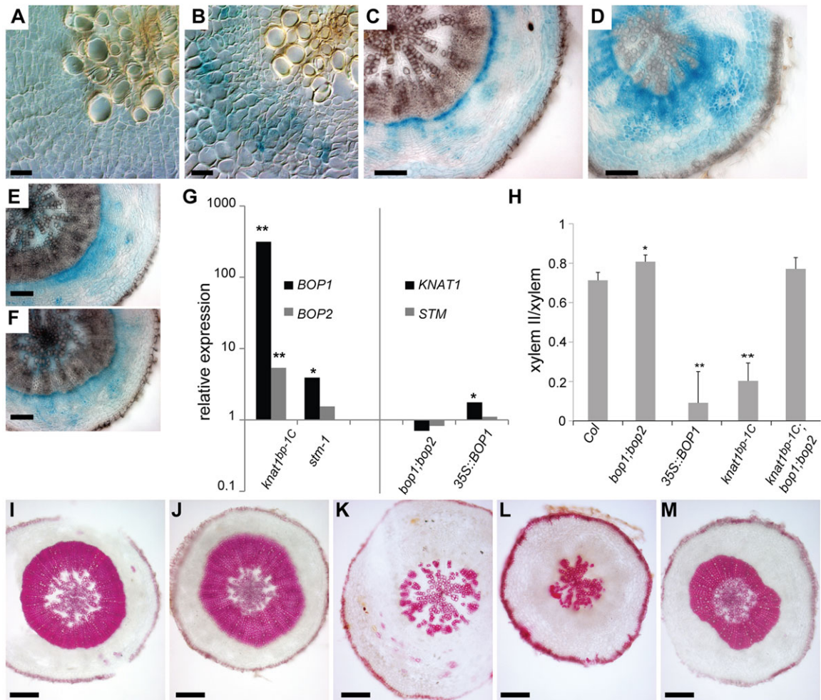
Fig. 8. KNAT1 and STM regulate xylem fiber differentiation through BOP1 and BOP2 . (A–F) GUS reporter activity in transverse sections of 3-week-old (A, B) and 5-week-old (C–F) hypocotyls. (A) p BOP1 ::GUS; (B) p BOP1 ::GUS; knat1 bp-1C ; (C) p BOP2 ::GUS; (D) p BOP2 ::GUS; knat1 bp-1C ; (E) p KNAT1 ::GUS; (F) p KNAT1 ::GUS; bop1;bop2 . (G) qRT-PCR experiments employed RNA of 4-week-old hypocotyls from three different independent experimental replicates. Data represent averages of experimental replicates. Expression is relative to ACT2 and normalized to expression in Col-0 (=1). (H) Ratio between the area occupied by xylem II and total xylem in transverse sections from 6-week-old hypocotyls. Data are mean±s.d. of three independent experiments per genotype, with three hypocotyls per experiment. (G, H) * P < 0.05 ; ** P < 0.01 , t -test comparing mutants with wild type. (I–M) Phloroglucinol staining of 6-week-old hypocotyls: (I) wild type (Col-0); (J) bop1;bop2 ; (K) 35S::BOP1 ; (L) knat1 bp-1C ; (M) knat1 bp-1C ; bop1;bop2 . Scale bars: 20 \mu m in A, B; 100 \mu m in C–F; 200 \mu m in I–M.
