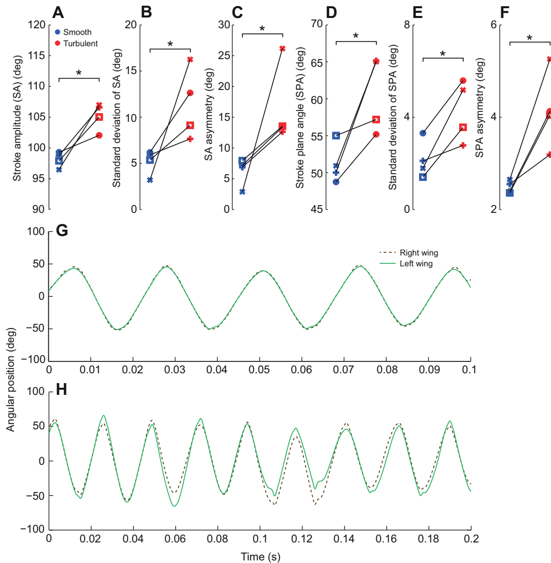
Fig. 6. Wing kinematic parameters during flight in smooth and turbulent flow. (A) Mean, (B) standard deviation and (C) mean bilateral asymmetry of stroke amplitude in smooth (blue) and turbulent (red) flow. (D) Mean, (E) standard deviation and (F) mean bilateral asymmetry of anatomical stroke plane angle in smooth (blue) and turbulent (red) flow. (G,H) Sample time traces of left and right wing sweep position during flight in (G) smooth and (H) turbulent flow, demonstrating increased wing asymmetry during flight in turbulence.
