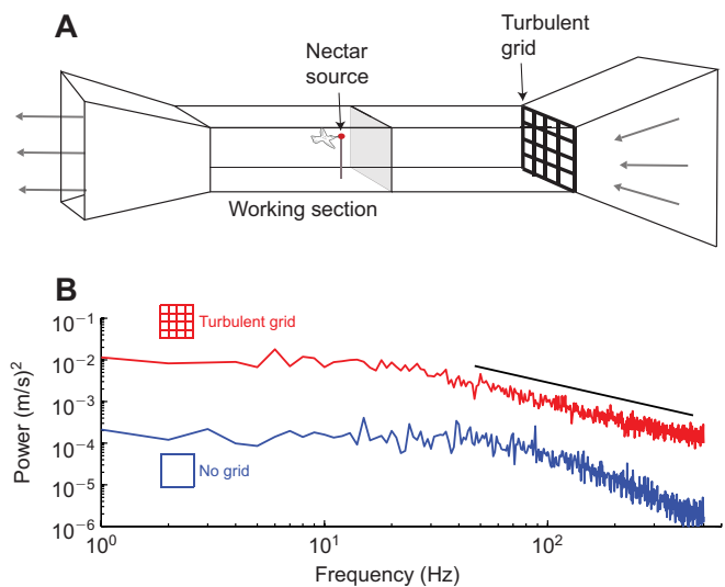
Fig. 1. Schematic diagram of the wind tunnel and power spectral density of wind in smooth and turbulent conditions. (A) Schematic diagram of the wind tunnel with a planar turbulence grid placed at the inlet of the test section. A screen (gray square) was placed upstream of the nectar source to prevent the birds from flying into the contraction section of the wind tunnel, and all airflow measurements were taken downstream of the screen and feeder. Arrows indicate wind direction. (B) Power spectral density of velocity fluctuations in smooth and turbulent wind conditions. Black line indicates a slope of -5/3 , a distinguishing characteristic for fully mixed freestream turbulence.
