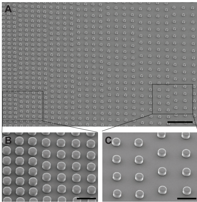
Fig. 1. Scanning electron microscope micrographs of the transparent ‘gradient’ microstructured epoxy substrate with square arrays of cylindrical pillars 1.4 \mu\text{m} in height and 2 \mu\text{m} in diameter. (A) From left to right, the centre-to-centre spacing increases from 3.5 to 6.5 \mu\text{m} in steps of 0.5 \mu\text{m} . (B) Transition from 3.5 to 4.0 \mu\text{m} spacing. (C) Transition from 6.0 to 6.5 \mu\text{m} spacing. Scale bars: 20 \mu\text{m} in A, and 5 \mu\text{m} in B,C.
