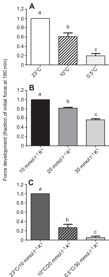
Fig. 4. Tetanic force production at combinations of different temperatures and [K + ] o with TTX present. (A) Tetanic force production measured at 23, 10 and 0.5°C. Force production at the different temperatures is normalized to force at 23°C. (B) Tetanic force production measured at 10, 20 and 30 mmol l -1 K + . Force production at the different potassium concentrations is normalized to force at 10 mmol l -1 . (C) Tetanic force production measured at combinations of lowered temperature and increased [K + ] o (23°C/10 mmol l -1 K + , 10°C/20 mmol l -1 K + and 0.5°C/30 mmol l -1 K + ). Force production at the different combined treatments is normalized to force at 23°C/10 mmol l -1 K + . All treatments were performed on TTX-treated preparations. Bars represent means ± s.e.m. of five to seven preparations in each treatment. Different letters indicate groups that differ significantly.
